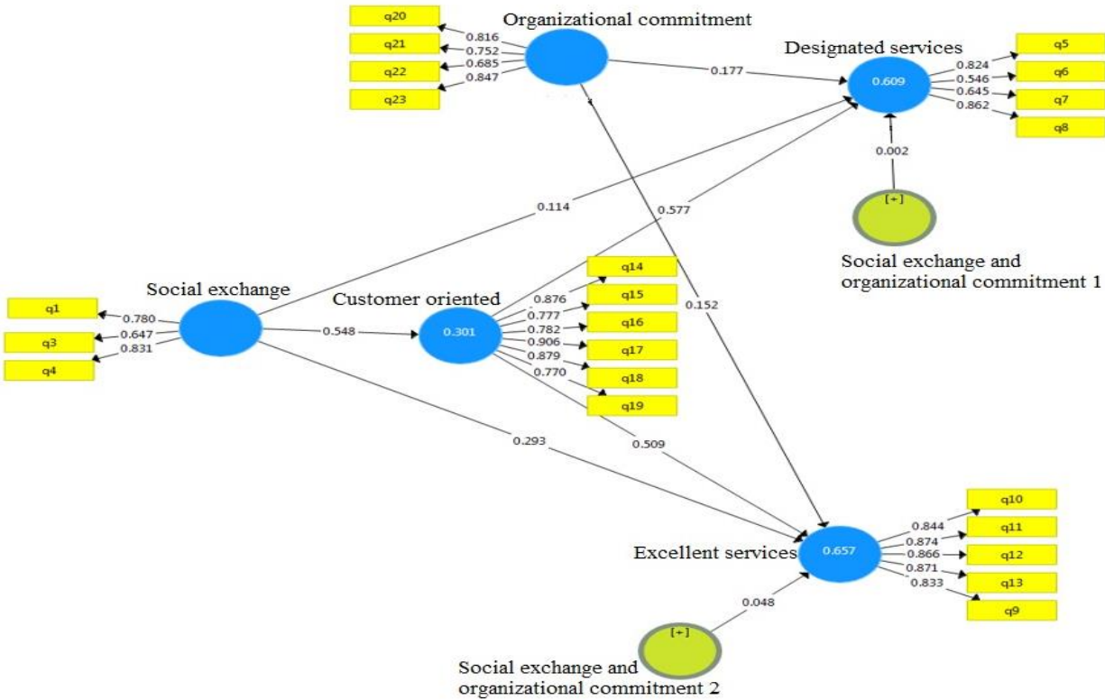
Figure 1: Coefficients of factor loads
